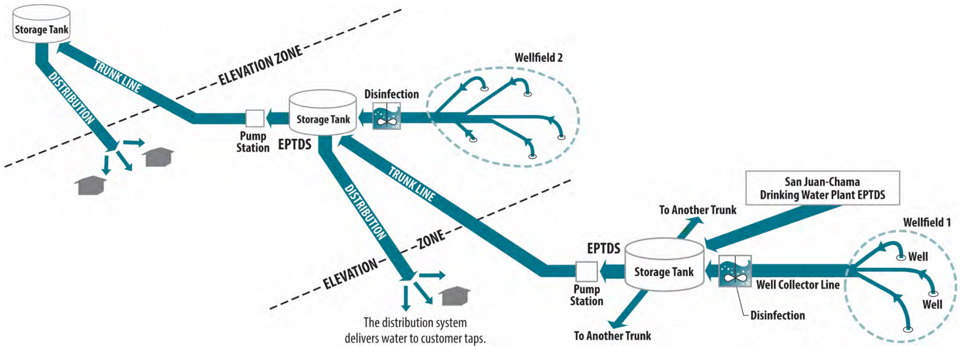
Figure 4 Entry Points to the Distribution System
